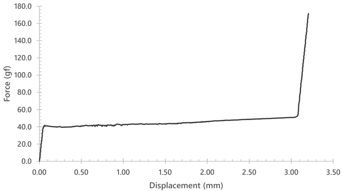
Haimu Sunny Clipper (Upstroke)
